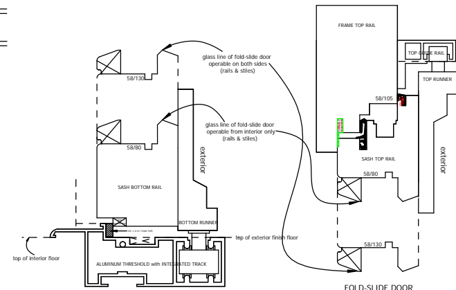
FOLD-SLIDE DOOR OUTSWING, BOTTOM HUNG ALL ALUMINUM THRESHOLD WITH INTEGRATED TRACK
