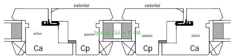
FOLD-SLIDE, INSWING, MEETING STILES "C"
