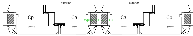
FOLD-SLIDE, OUTSWING, MEETING STILES "C"
