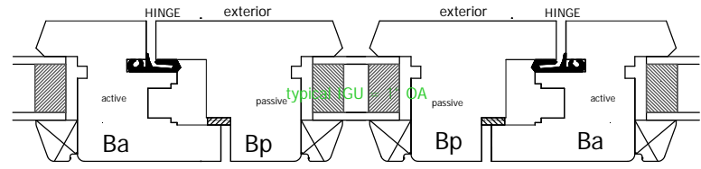
FOLD-SLIDE, INSWING, MEETING STILES "B"
