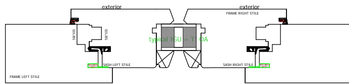
FOLD-SLIDE, OUTSWING, LEFT & RIGHT STILES
