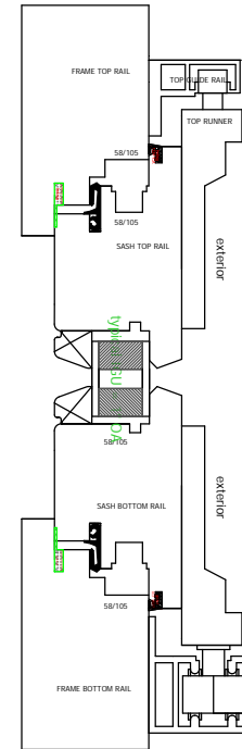
FOLD-SLIDE WINDOW, OUTSWING, BOTTOM HUNG
