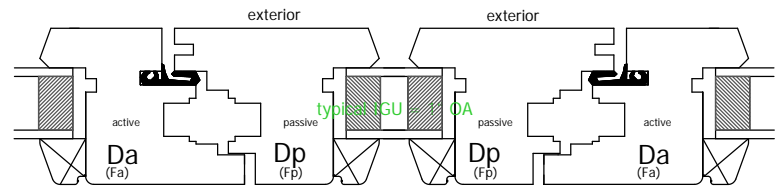
FOLD-SLIDE, INSWING, MEETING STILES "D"
