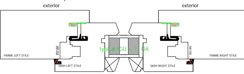
FOLD-SLIDE, INSWING, LEFT & RIGHT STILES
