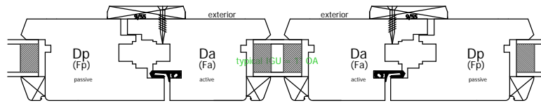
FOLD-SLIDE, OUTSWING, MEETING STILES "D"
