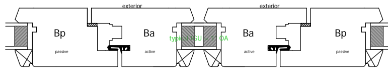
FOLD-SLIDE, OUTSWING, MEETING STILES "B"
